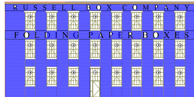
10 PROPOSED SIDE ELEVATION SCALE: 1/8" = 1'-0"
