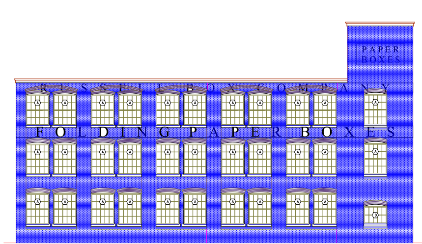
7 PROPOSED REAR ELEVATION SCALE: 1/8" = 1'-0"
