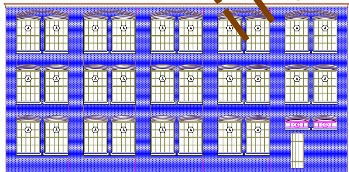
5 PROPOSED FRONT ELEVATION SCALE 1/8" = 1'-0"
