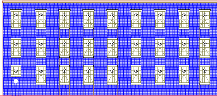
1 PROPOSED FRONT ELEVATION SCALE 1/8" = 1'-0"
