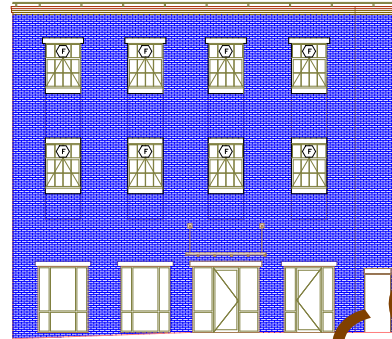
3 PROPOSED FRONT ELEVATION SCALE 1/8" = 1'-0"
