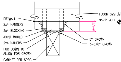
SECTION THRU SOFFIT
