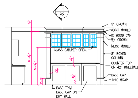
PSO-4 KITCHEN ELEVATION
