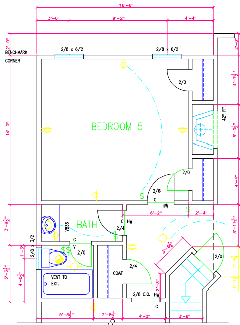
PSO-1 OPTIONAL 5th BEDROOM & FULL BATH
