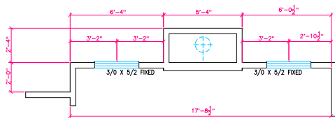
OPT. REAR FIREPLACE UPPER LEVEL
