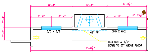
PSO-2 OPT. REAR FIREPLACE
