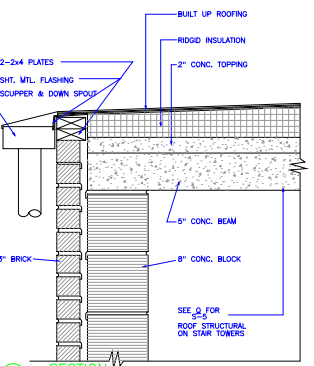
6 AS SECTION SCALE 1-1/2" = 1'-0"
