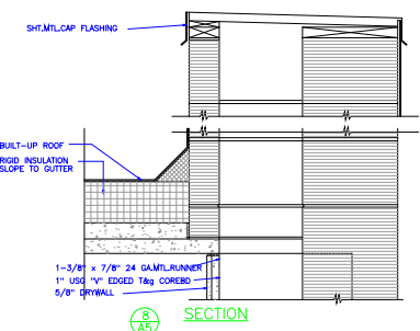
8 AS SECTION
