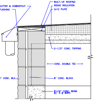
5 AS SECTION SCALE 1-1/2" = 1'-0"
