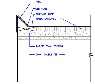
4 AS SECTION SCALE 1-1/2" = 1'-0"
