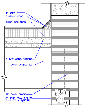
2 AS SECTION SCALE 1-1/2" = 1'-0"
